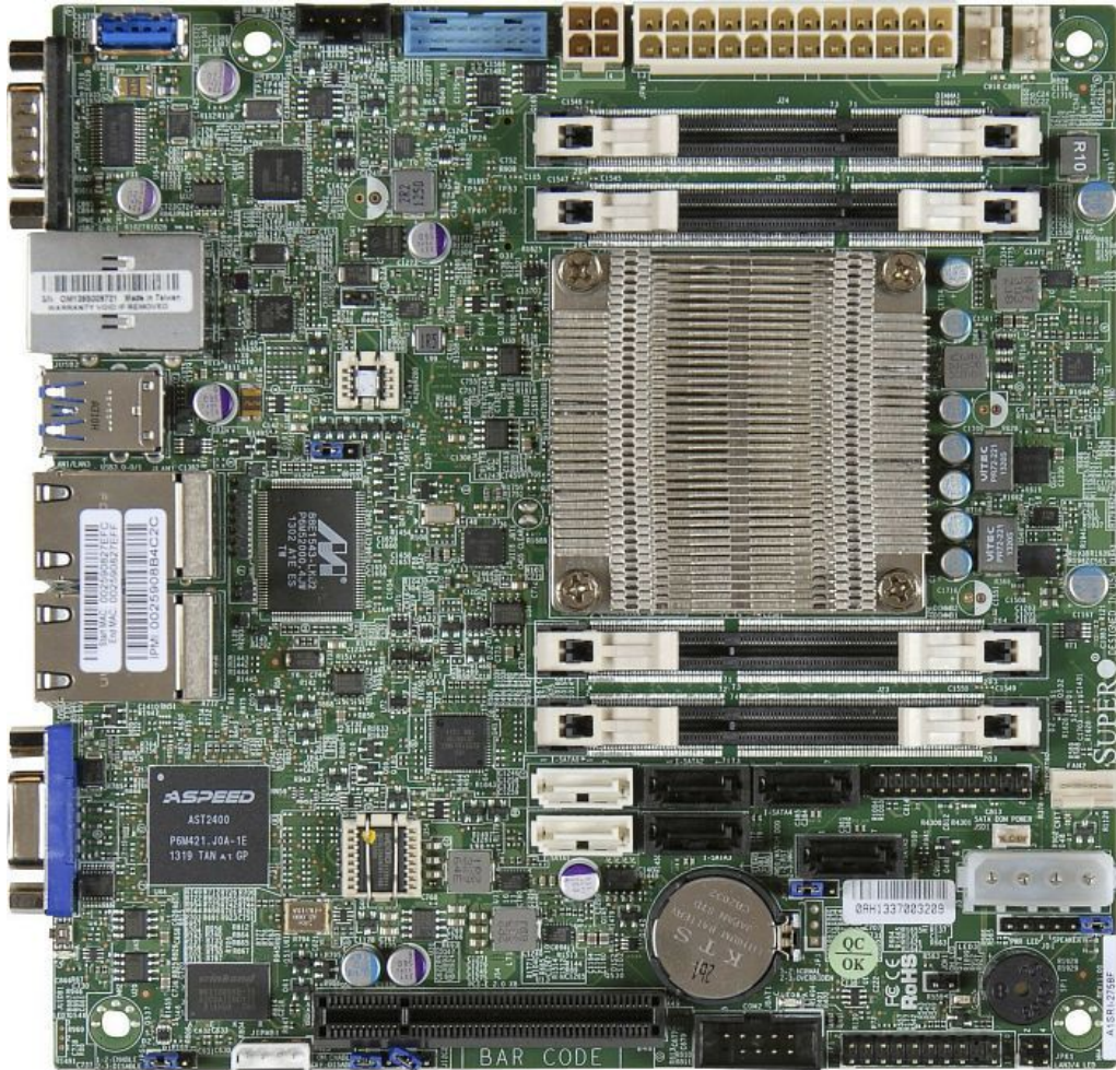
Figure 5: Super Micro A1SAi-2550F top view
